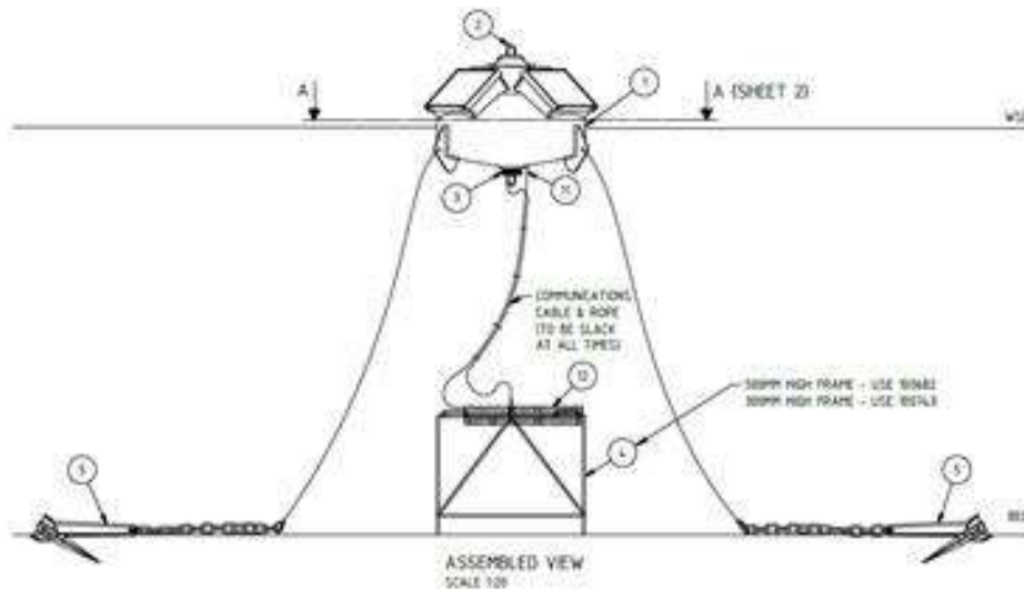
Figure 2: SEA 170 Buoy
